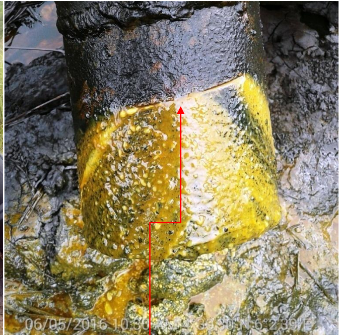
Fig B: The leak point (Hacksaw cut)
